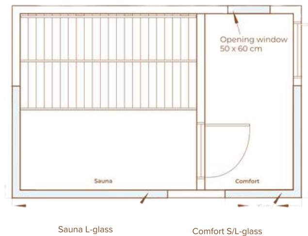
TAVO Sauna Comfort S
