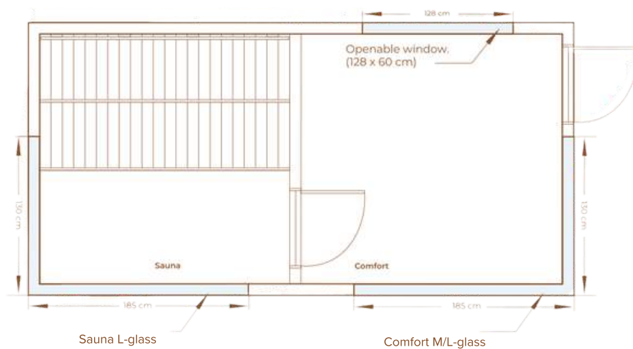
TAVO Sauna Comfort M
