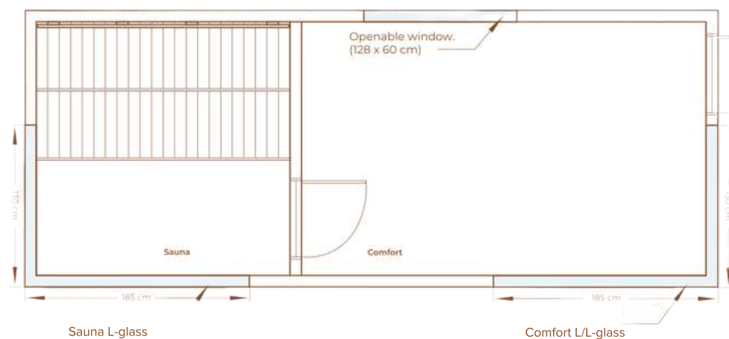
TAVO Sauna Comfort L
